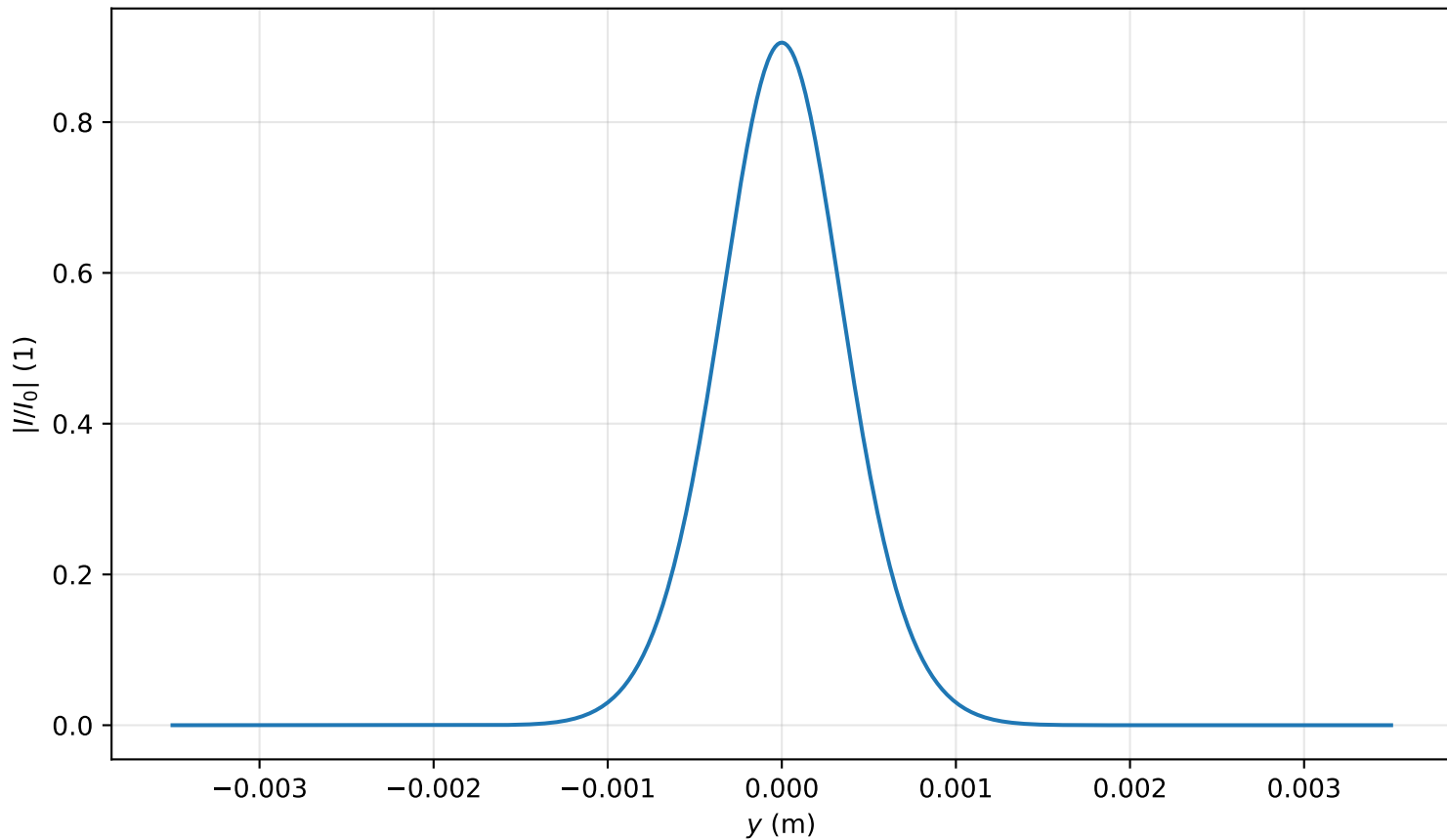
Intensity profile I(x = 0, y, z = 1.115)/I_0 , P_{in}=0.3P_{cr} , artificial time
